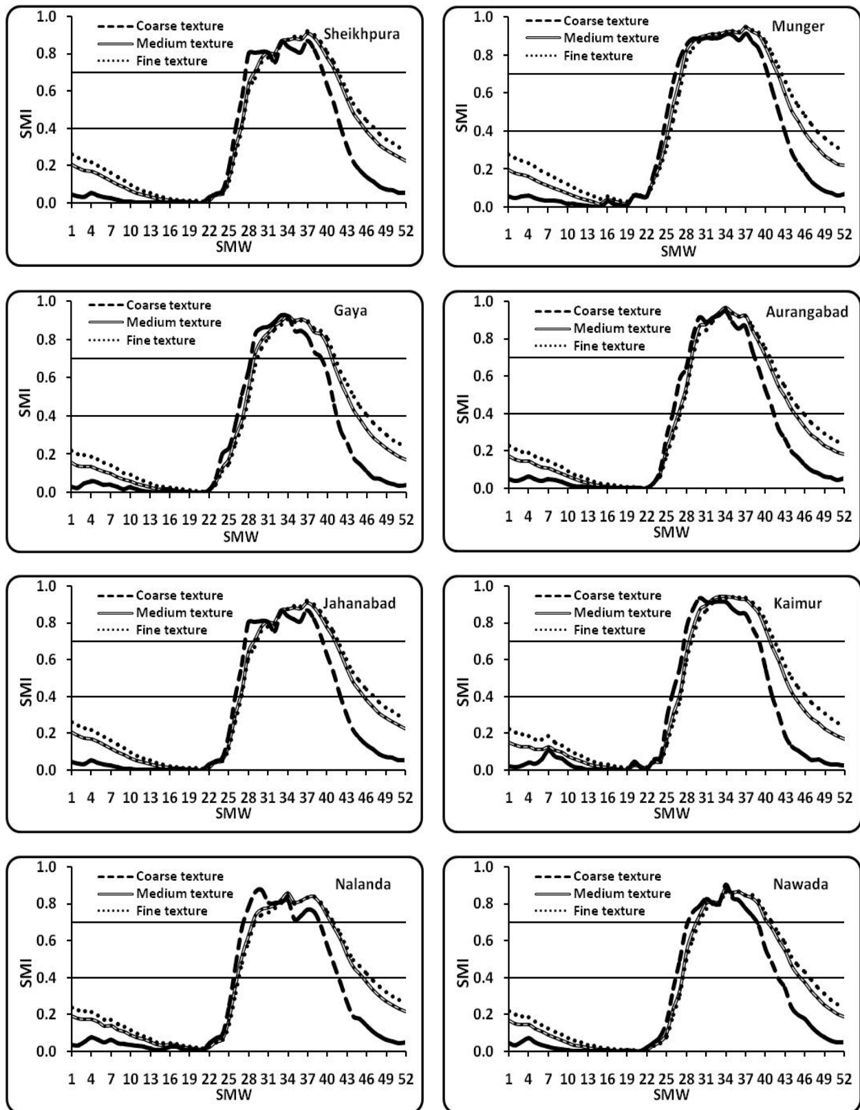
Fig. 6. Variation in weekly soil moisture index (SMI) in Zone IIA (Sheikhpura and Munger districts) and Zone IIIB (Gaya, Aurangabad, Jahanabad, Kaimur, Nalanda and Nawada districts)
