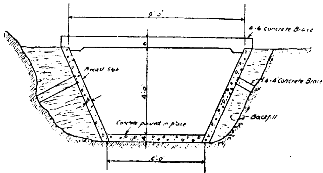
CROSS SECTION OF DITCH
