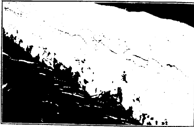
FIG. 4. Chicken wire and concrete plaster lining damaged by erosion and temperature cracks.
